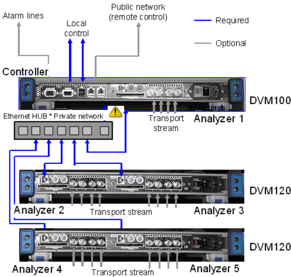
Figure 2-10: Connections of an R&S DVM100L + R&S DVM120 basic configuration
