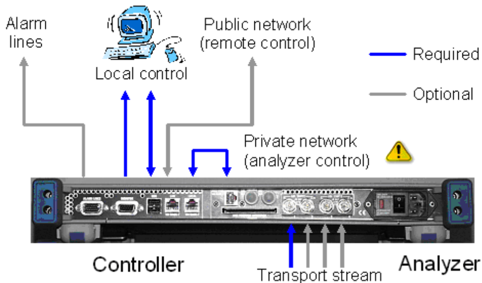
Figure 2-9: Connections of basic configuration of R&S DVM100L
